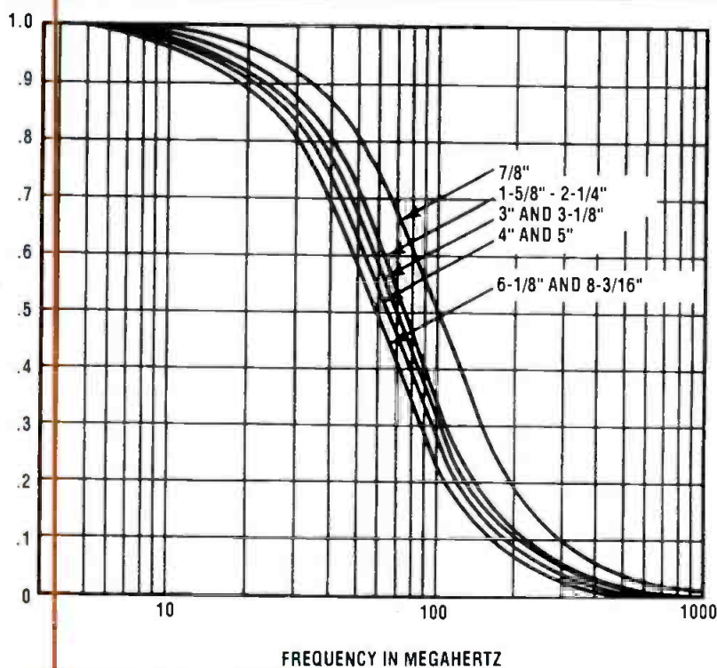
3. Derating factor for average power due to VSWR. High VSWR reduces the power-handling capability of transmission lines.
