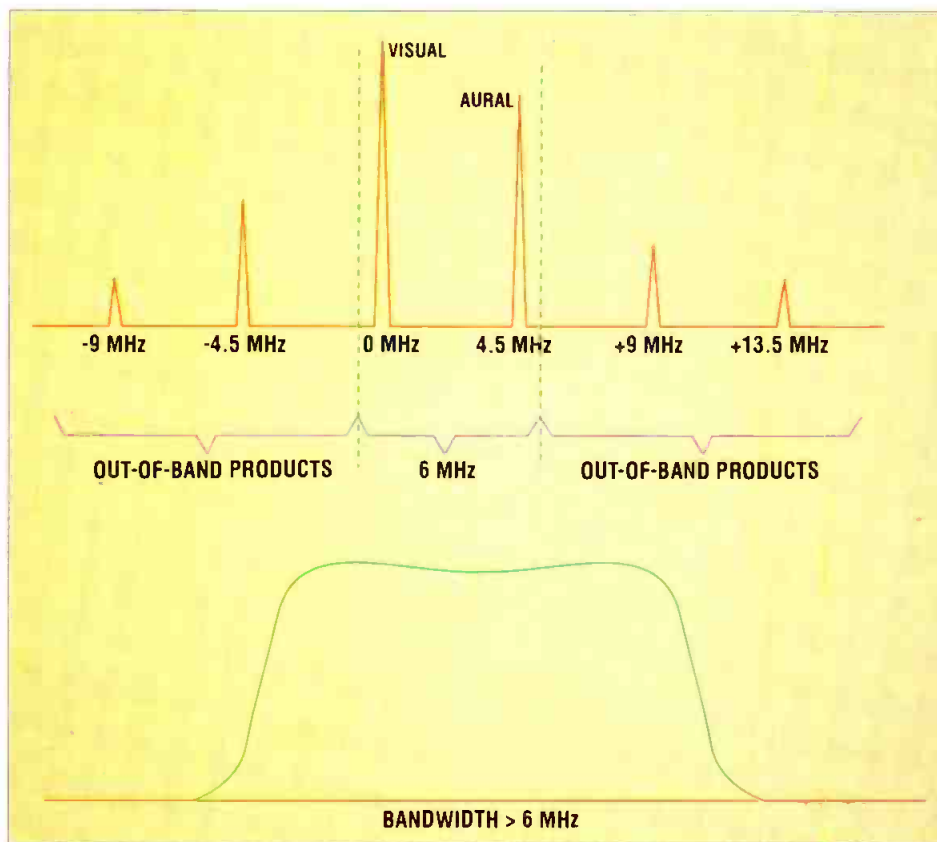
Figure 1. Typical analog measurements ignore the IM that occurs in adjacent channels because proper filtering can eliminate them.
