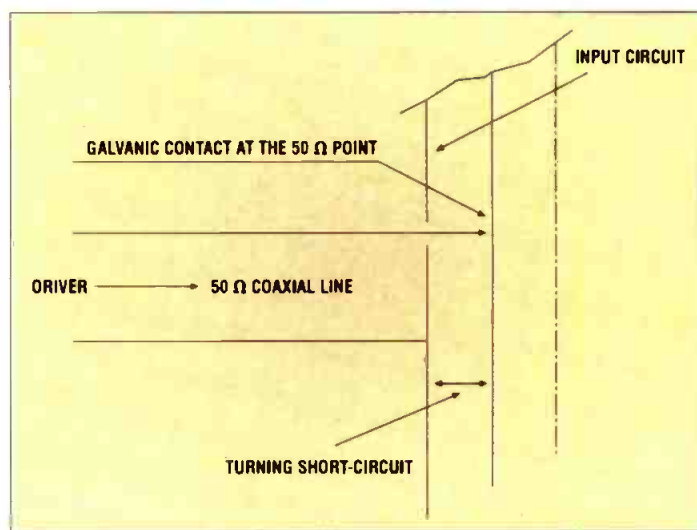
Figure 6. Tubes such as the tetrode, Diacode and IOT rely on a wideband galvanic coupling at the 50Ω point in the input cavity.
