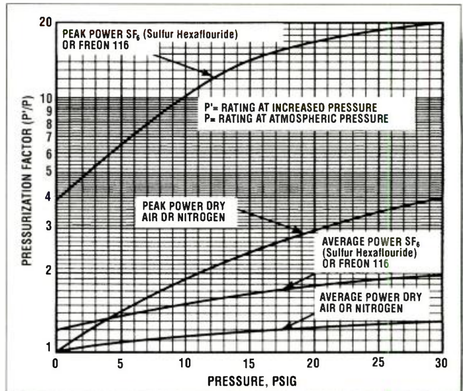
Figure 1. Pressurization factors, 50Ω line. It's easy to pump more through your line, just use more pressure, but, be careful; the loss of pressure or the use of \text{SF}_6 gas or Freon 116 carry their own operational cost penalties.
